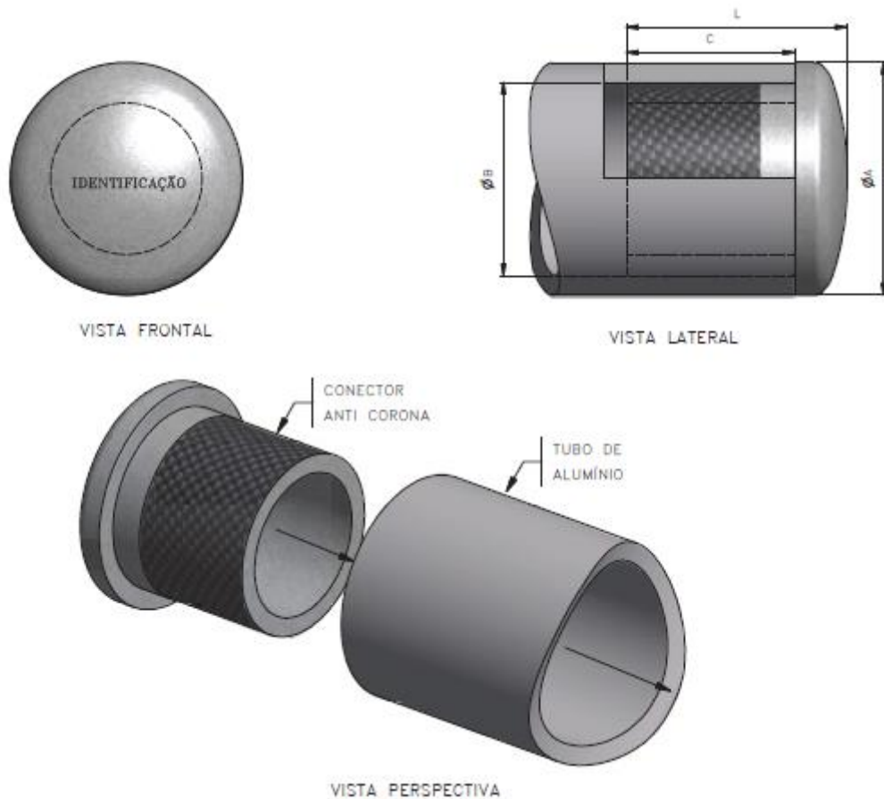
Figura 1 - Conector Anti-corona
