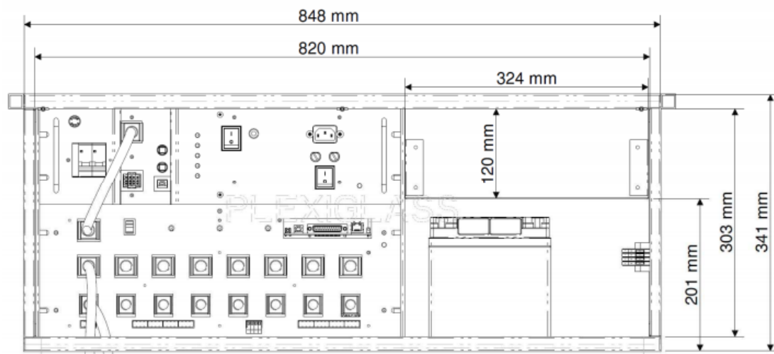
Figure 11 Ë Front view of the indoor CM-UP Cabinet container, quotes are indicative: must be guaranteed compatibility with the CM-UP support, figure 11
