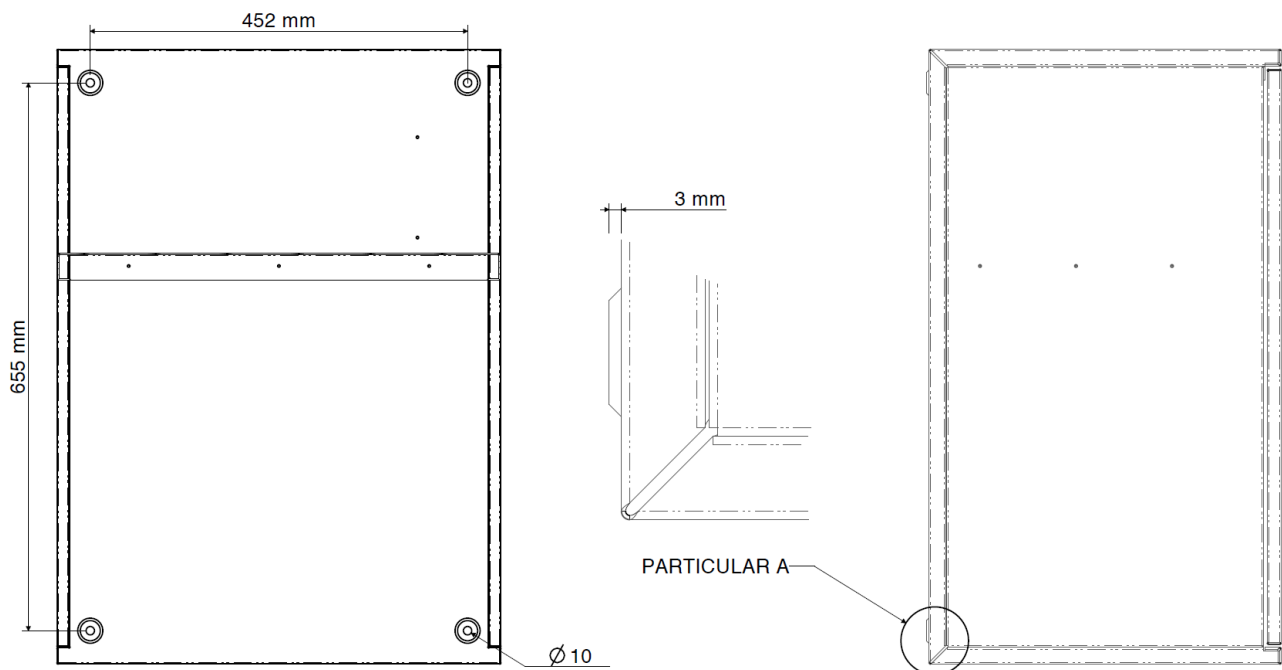
Figure 16 Ě wall-mounting details
