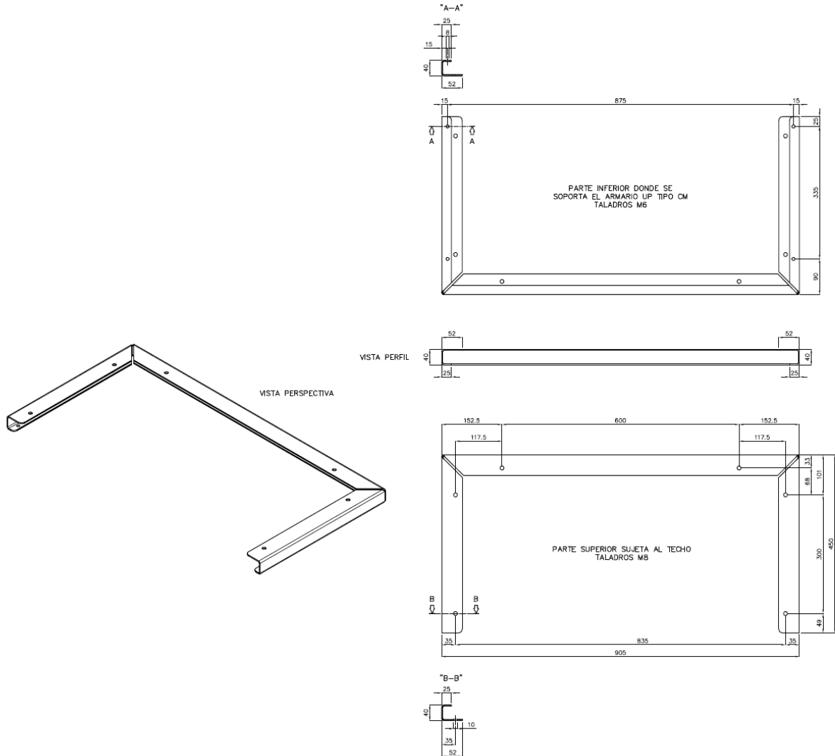
Figure 13 – CM-UP dimensions, to guarantee interchangeability
