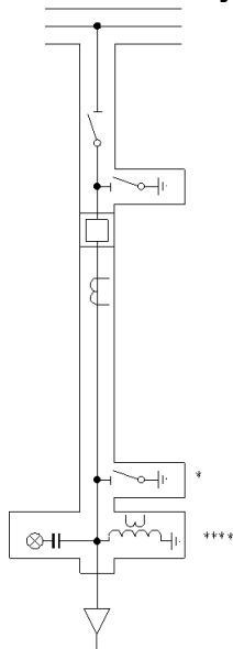
Transformer bay
