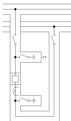
Coupling bay
