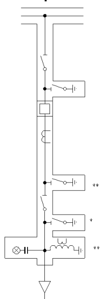
Output or Self-producer bay
