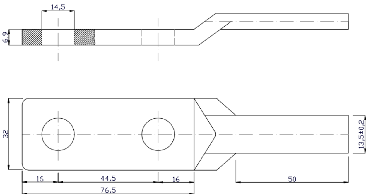
Figura 1 – Conector terminal barra chata com 2 furos
