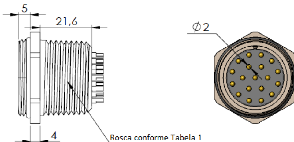
Figura 1 – Conector TCM
